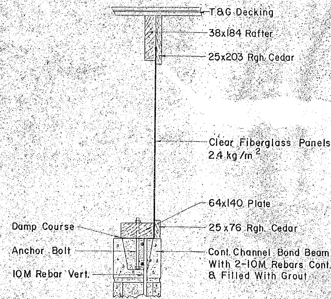
DETAIL 'C'
