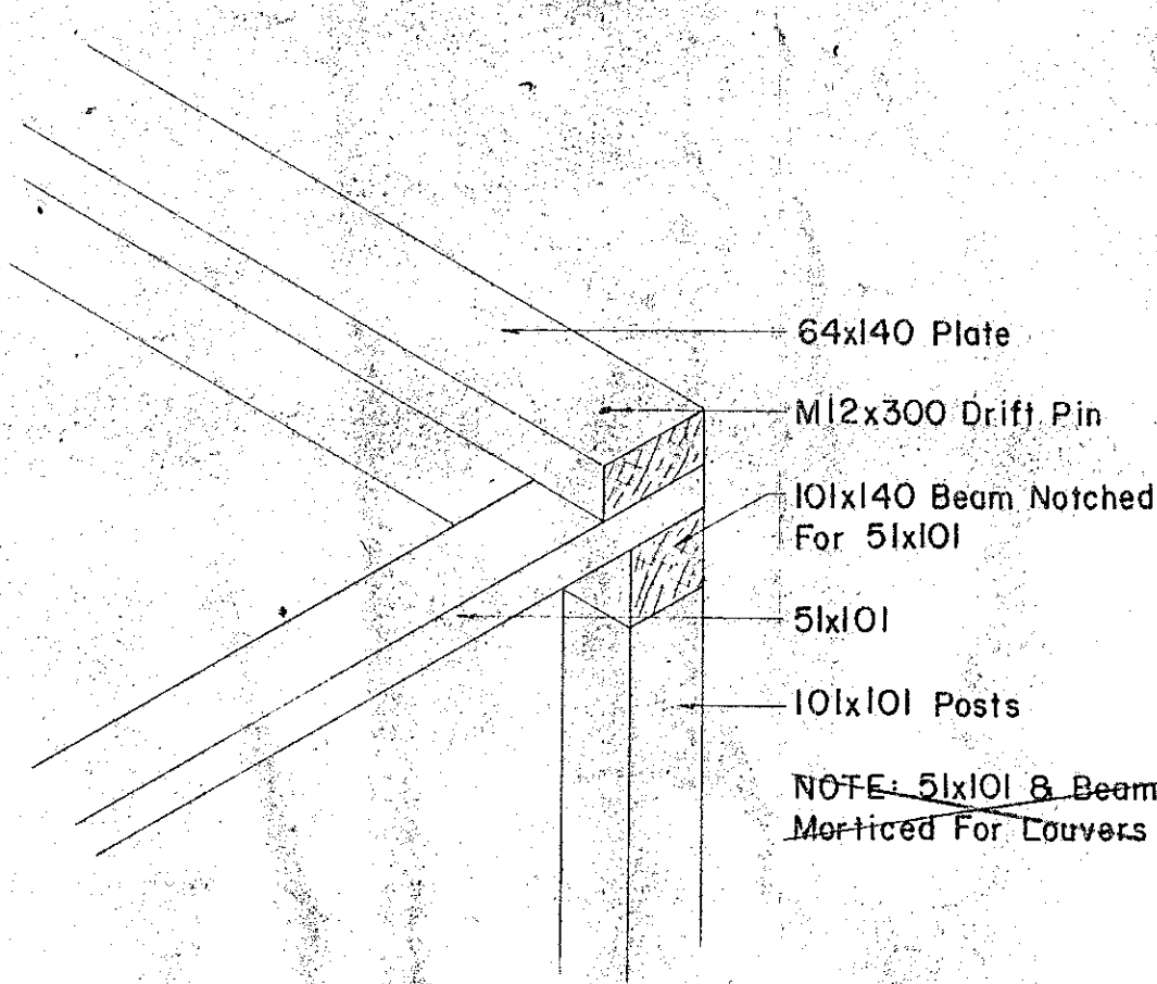
DETAIL 'A'
